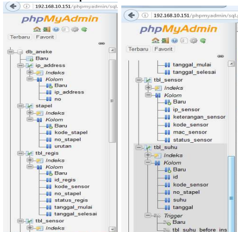
Gambar 13. Database Server
