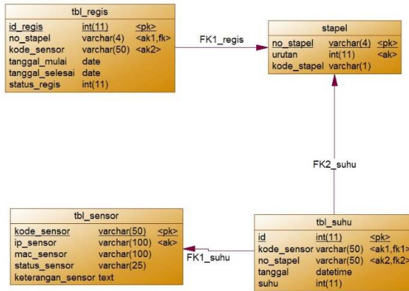
Gambar 12. Physical Data Model
