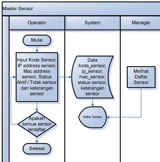
Gambar 5. System flow Master Sensor
