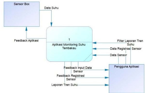
Gambar 10. Context Diagram
