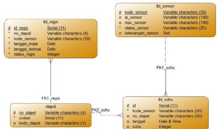
Gambar 11. Conceptual Data Model
