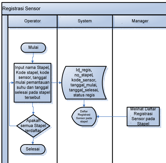
Gambar 6. System Flow Registrasi Sensor
