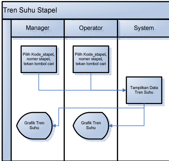
Gambar 8. System Flow Tren Suhu stapel
