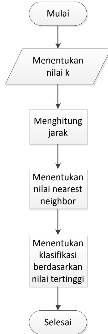
Gambar 1 Flowchat k-NN
